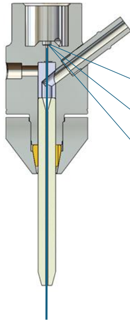
Abrasive diamond head
